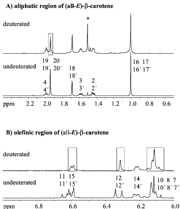
Figure 6. ^1\text{H} NMR spectra (600 MHz, 5 mm tube) of synthetic labeled ^2\text{H}_8 -( all-E )- \beta -carotene and unlabeled standard in chloroform- ^2\text{H}_1 . (A) Aliphatic region of ( all-E )- \beta -carotene, with the lower spectrum depicting undeuterated and the upper spectrum depicting deuterated ( all-E )- \beta -carotene. (B) Olefinic region of ( all-E )- \beta -carotene, with the lower spectrum depicting undeuterated and the upper spectrum depicting deuterated ( all-E )- \beta -carotene (* interfering signals).
