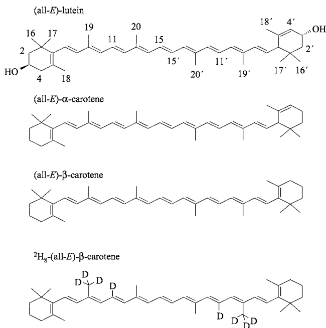
Figure 1. Chemical structures of ( all-E )-lutein, ( all-E )- \alpha -carotene, ( all-E )- \beta -carotene, and ^2\text{H}_8 -( all-E )- \beta -carotene.
