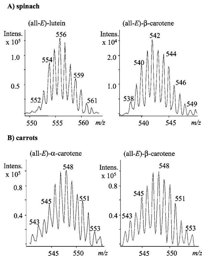
Figure 3. The Gaussian isotopomer distribution of the deuterated ( all-E )-lutein and ( all-E )-β-carotene from labeled spinach (A) and ( all-E )-α-carotene and ( all-E )-β-carotene from labeled carrots (B).
